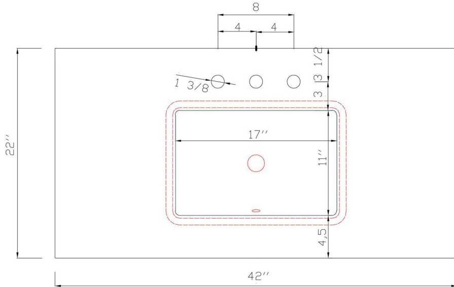
TOP VIEW
