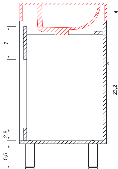
A - A SECTION
