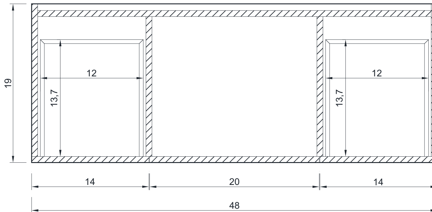
C - C SECTION
