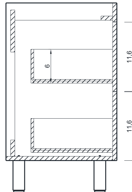
B - B SECTION
