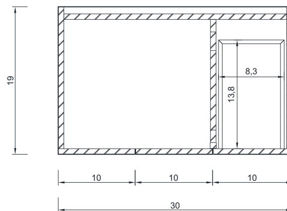
C - C SECTION
