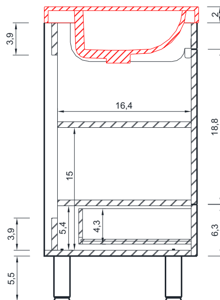
A - A SECTION
