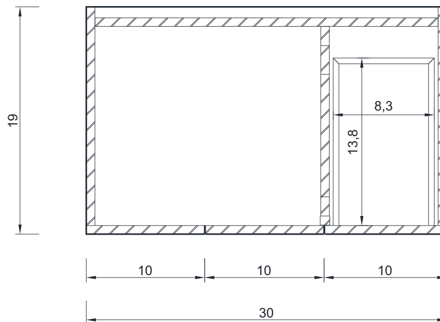
C - C SECTION
