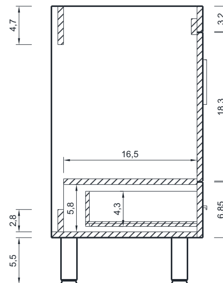
A - A SECTION
