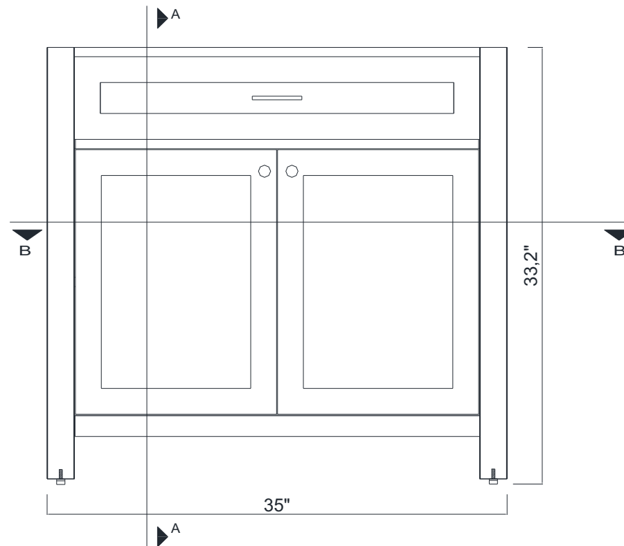
Vanity Without Top
