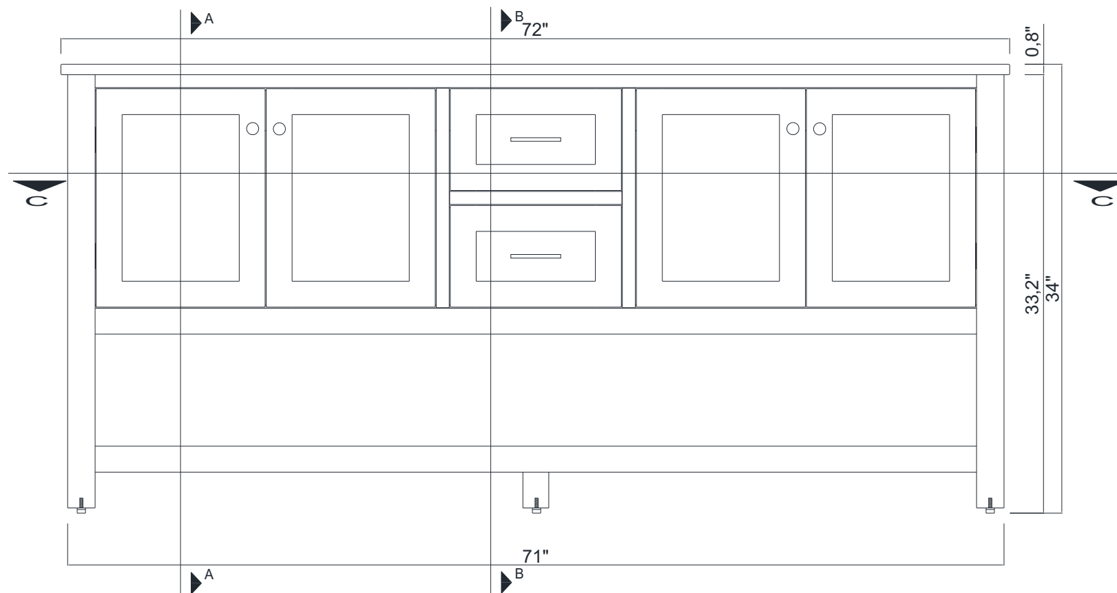
FRONT VIEW
